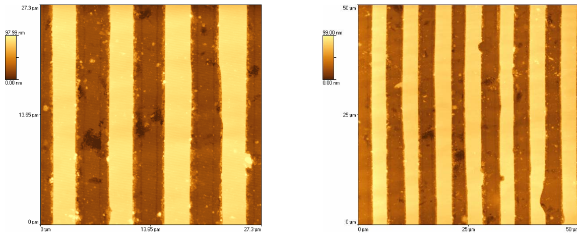
Fig. 6. Scanning probe microscopy observation of the periodical domain structure revealed by etching in 0.5 mm thick MgO:LN
