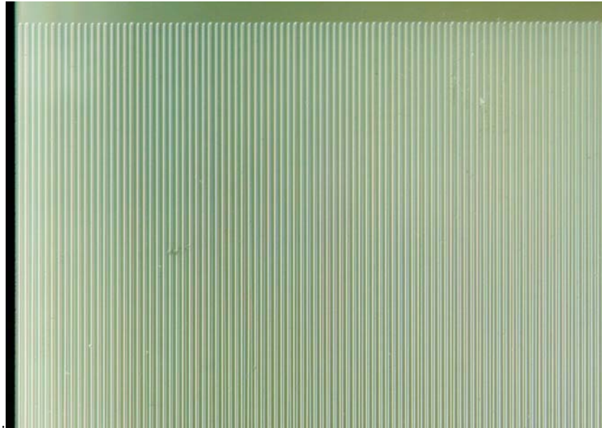
Fig. 5. Optical microscopic image of the etched PP structure for the 0.5 mm thick PPLN element with a 6.78 \mu\text{m} domain inverted period on Z+ surface.
