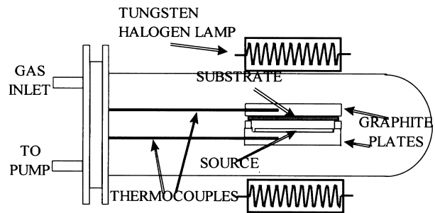
Fig. 2. Schematic diagram of CSS deposition chamber.
